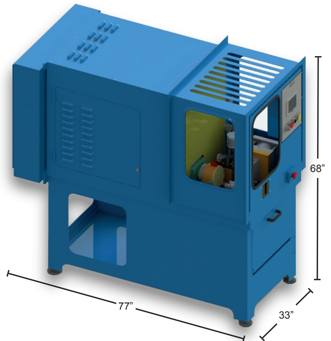
Model 21HY Footprint 33"W x 77"D x 68"H
